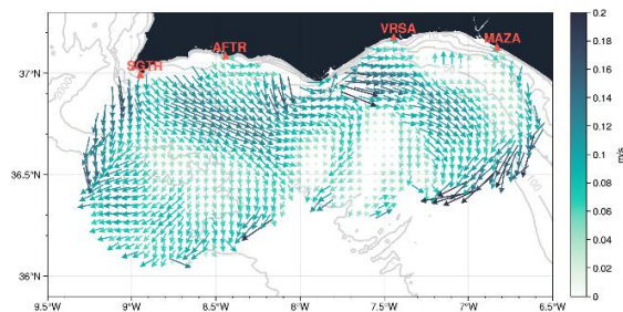
Figure 2. Surface current vectors (colored by magnitude) from the HFR-South network. Red markers indicate antennae locations: SGTR (Sagres), AFTR (Alfanzina), VRSA (Vila Real de Santo António), and MAZA (Mazagón).
