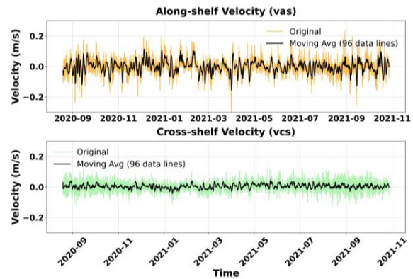
Figure 3. Time-series of along-shelf (top) and cross-shelf current velocity components for the entire measurement period (from August of 2020 to October of 2021) at 2.75 m from the bottom. The above bar represents the timeline according to the time between the successive sampling campaigns. The colored lines in both plots represent the original measured values while the black lines represent the moving average with a window equal to 96 data lines (corresponding to one day of measurements).
