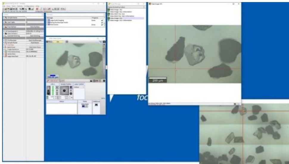
Figure 3. Search for sand target particles with the 10\times/0.25 magnification lens of the confocal Raman microscope WITec® alpha300 R system.
