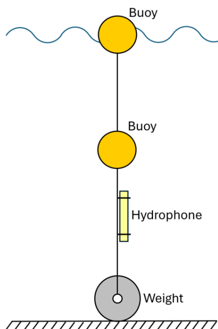
Figure 2. Diagram of the equipment used for hydrophone measurements.
