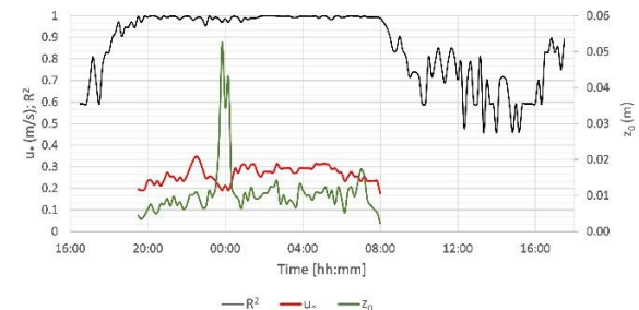
Figure 3. Time variation of R^2 (all data, grey line), z_0 (green line) and u^* (red line).
