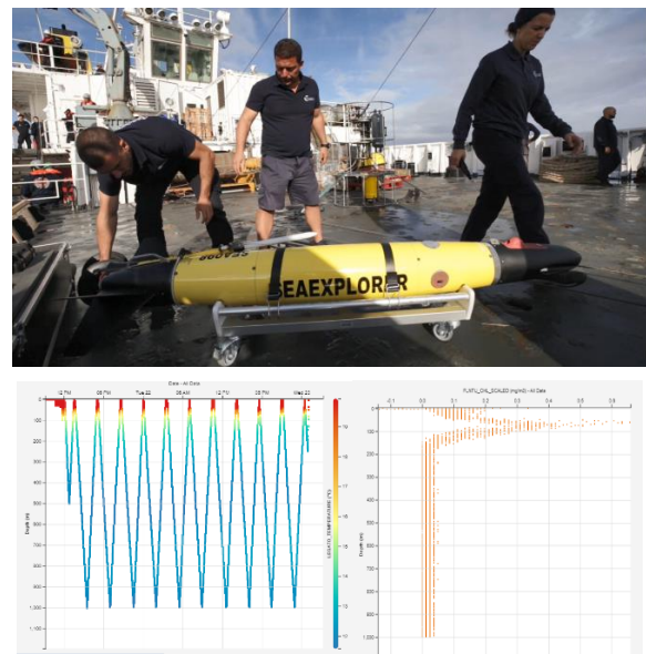
Figure 2. (Top) The IH glider onboard NRP D.Carlos I, being prepared for deployment. (Bottom left) Measurements of temperature along the track of the glider. (Bottom right) Ensemble of chlorophyll-a profiles for the overall section covered (bottom).
