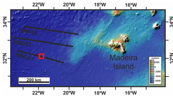
Figure 1. Location of multichannel seismic lines off Madeira Island. The red square indicates the location of seismic sections presented in Figure 2.
