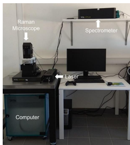
Figure 2. Confocal Raman microscope WITec® alpha300 R system at EEMT, IPMA Tavira.
