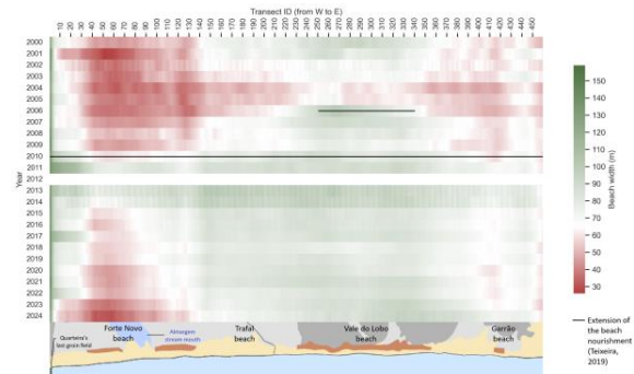
Figure 2. Evolution of the average annual width (m) of the study area, from 2000 to 2024, along the transects drawn every 10 m. The black lines indicate the extent of the beach area that was artificially nourished.
