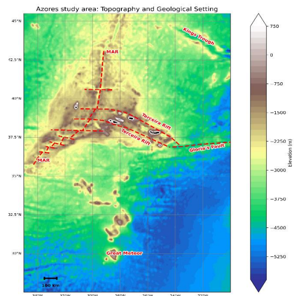
Figure 1. Topography and tectonic setting of the study area.
