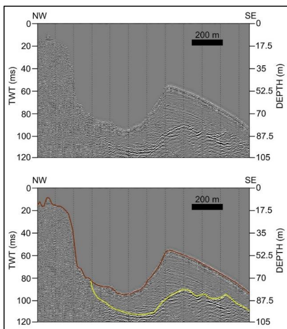
Figure 4. NW-SE-oriented Boomer seismic profile crossing the landslide scar. (A) Uninterpreted profile. (B) Interpreted profile, with the brown line indicating the seafloor and the yellow line outlining the basement.
