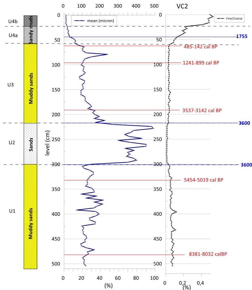
Figure 2. Along cores variability of mean grain size and mineralogical ratio (fine/coarse). Red lines represents the radiocarbon dating layers; and blue lines represents possible layers of 1755 and 3.6 cal BP tsunamis.
