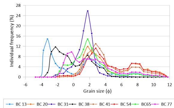
Figure 3. Grain size distribution.
