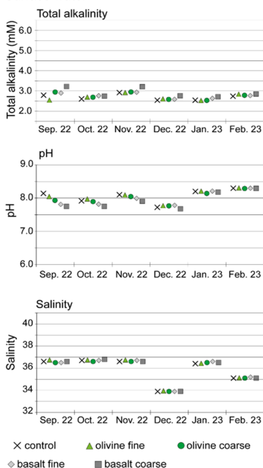
Figure 3. Records of total alkalinity, pH, and salinity measured in the surface water samples from plot 2, for the first 6 months of the experiment (adapted from Mendes et al. , 2025).
