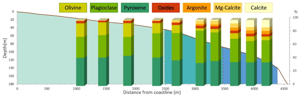
Figure 4. Spatial variation in the mineralogical composition of surface sediments along the cross-shore bathymetric profile.
