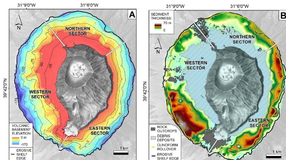
Figure 2. (A) Volcanic basement across the insular shelf. Thin dashed black contour lines are spaced every 25 m. (B) Sedimentary cover thickness (in m) of the insular shelf. Thin dashed blue isopaches are spaced every 10 m. The white lines delineate the boundaries between the shelf's sectors. Data in both maps are represented with cells size of 50 \text{ m}^2 .
