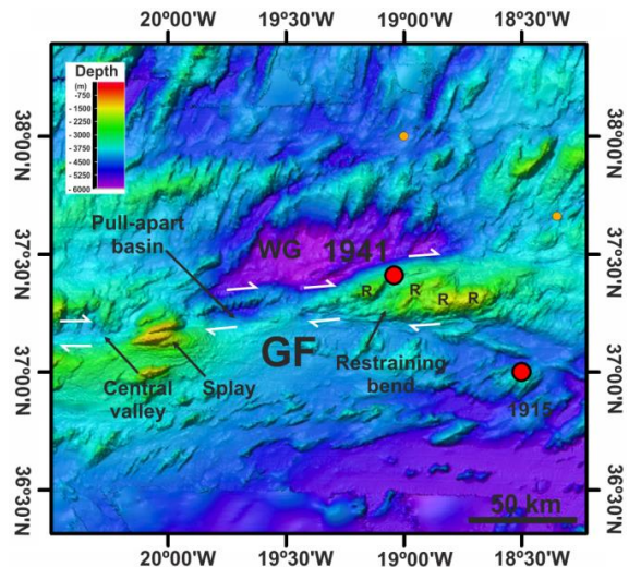
Figure 2. Multibeam bathymetry imaging the central segment of the Gloria Fault (GF) and showing the location of the 1941 earthquake epicenter (red dot) on top of a sigmoidal feature interpreted as a double restraining bend bounded by thrust-faults. WG: Western Gap; R: ridges.
