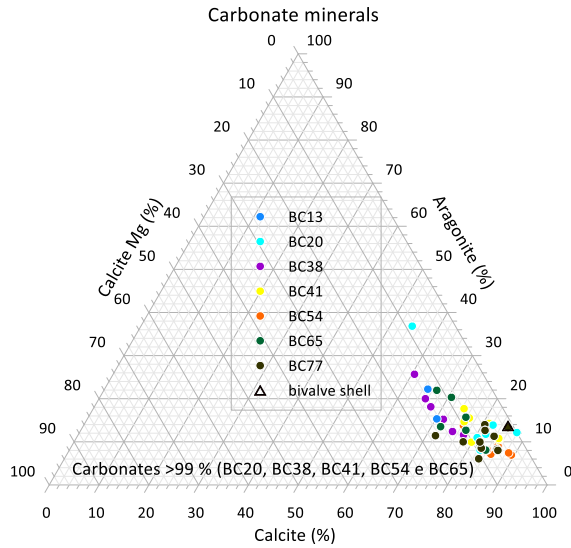
Figure 2. Ternary diagram showing the carbonate minerals of the analysed sediments, compared with XRD data from a bivalve shell. Intra and inter-BC variability can be observed.
