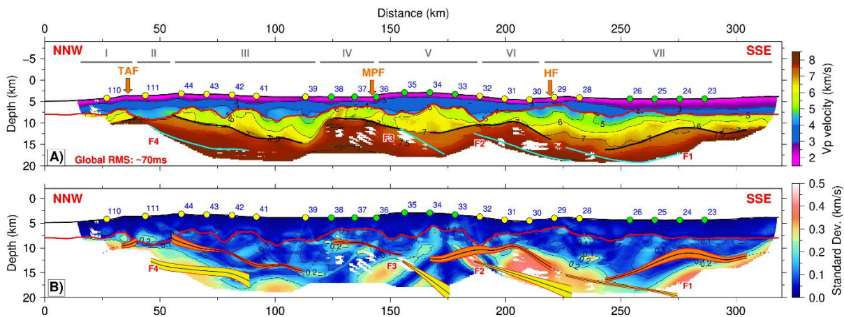
Figure. 2.(A) Final V_p Model for the profile P2AC1. The solid black and light-blue lines represent the Moho interface and the reflection planes of the potential faults respectively. (B) Standard deviation of V_p values of the average solution of the Monte-Carlo analysis for the profile P2AC1. The width of the red and yellow bands represents the standard deviation of the depth of the inverted horizons: Moho, F1, F2, F3 and F4. The circles on at the sea-bottom display the receiver locations: OBS (green) and OBH (yellow).
