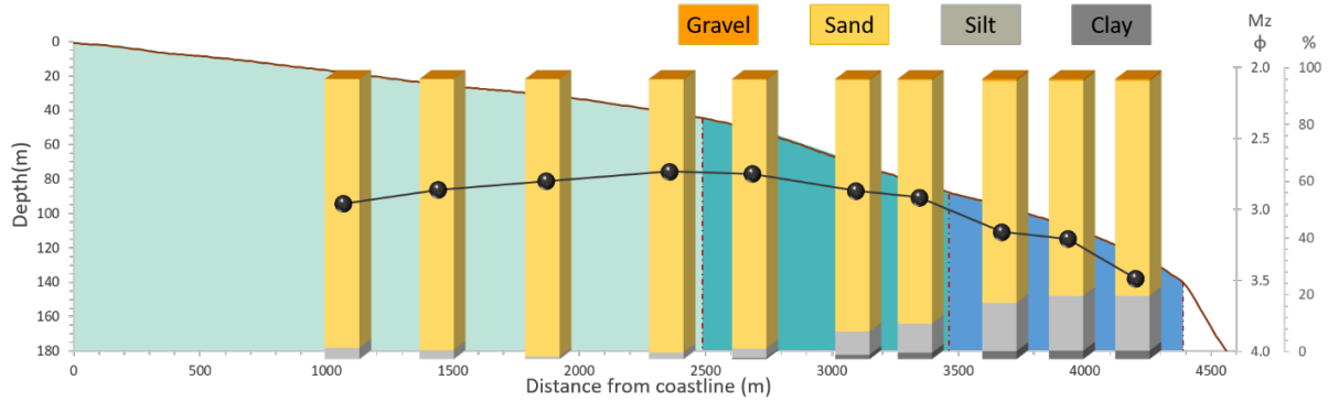
Figure 3. Spatial variation of the main textural classes and the mean grain size ( M_z ) of surface sediments along the cross-shore bathymetric profile.
