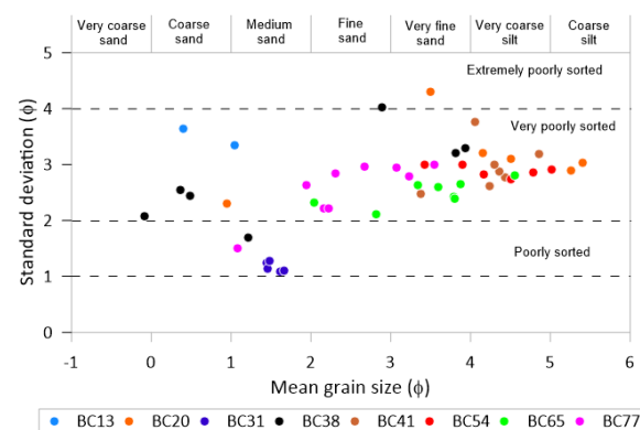
Figure 4. Relationship between the mean grain size and standard deviation.
