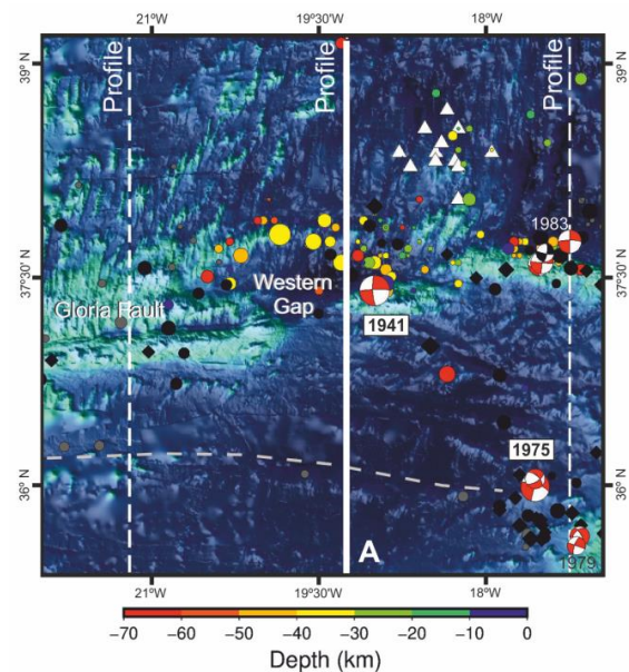
Figure 3. Map showing the location of epicenters and focal mechanisms of large earthquake in the study area, in particular of 1941 and 1979 events. White triangles correspond to the location of the DOCTAR experiment stations (Krüger et al. , 2020). The different colors correspond to the depth of the respective hypocenter. The gray dashed line represents the location of the Tydemán fracture zone. Straight vertical white dashed lines mark the location of bathymetric and depth across seismicity clusters. Profile A across the sigmoidal feature is shown in Figure 4.
