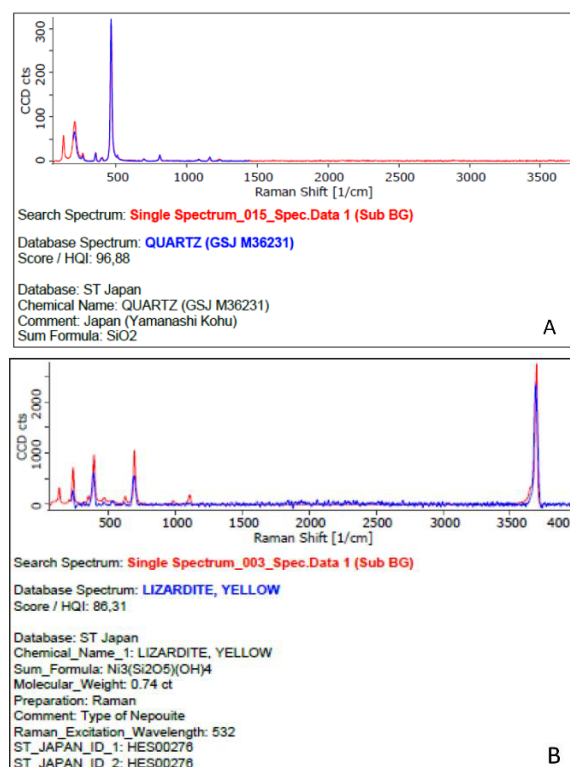
Figure 4. Two examples of the spectra obtained by micro-Raman analysis: A – grain from Tavira beach (Algarve); B - grain from the Estremadura Spur.
