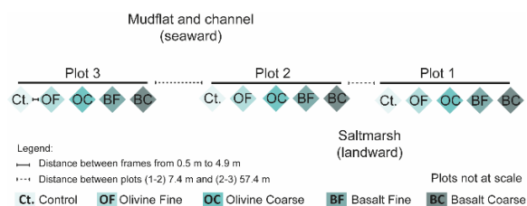
Figure 2. Schematic representation of the field experiment, composed by three plots, each one with the five experimental treatments installed in the salt marsh pioneer zone (adapted from Mendes et al. , 2025).
