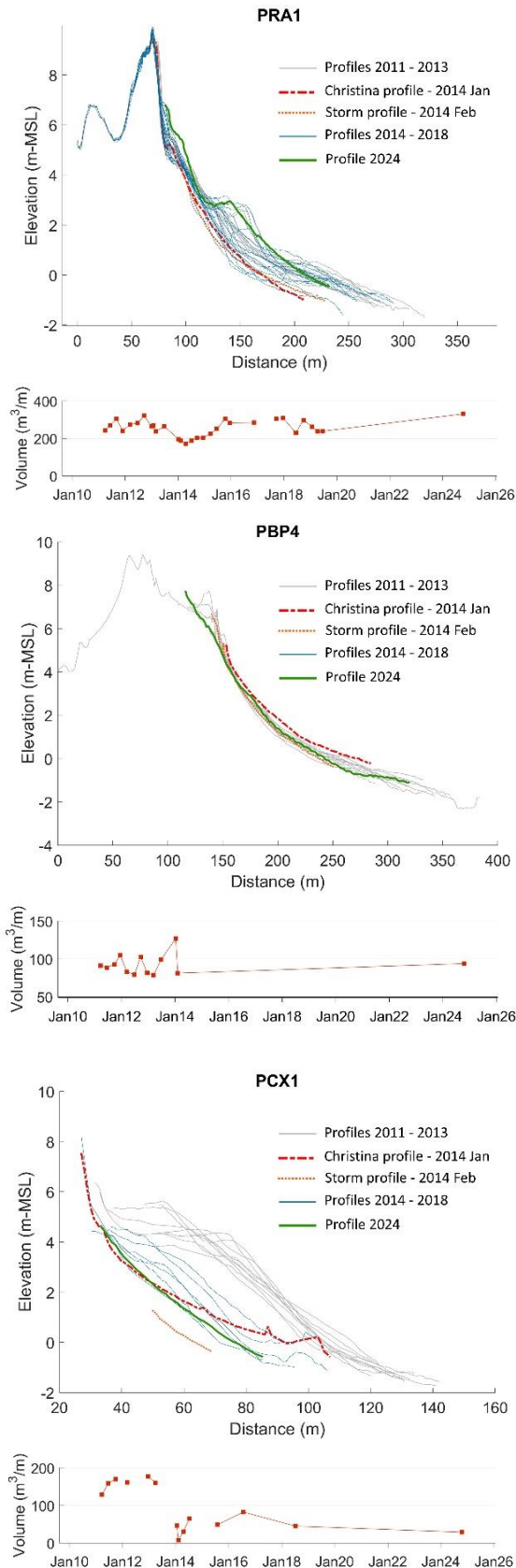
Figure 2. Beach profiles (Rainha beach - top panel; Baleal - Peniche sector - middle panel; Coxos beach - bottom panel) and variation in volumetric sediment retention: pre-Christina; aftermath of Christina, post-Christina recovery.
