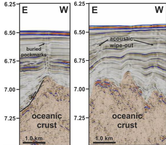
Figure 2. Sections of multichannel seismic line WM-01 showing evidence of fluid migration associated with basement highs. Vertical scale is in seconds TWTT. See Figure 1 for location.
