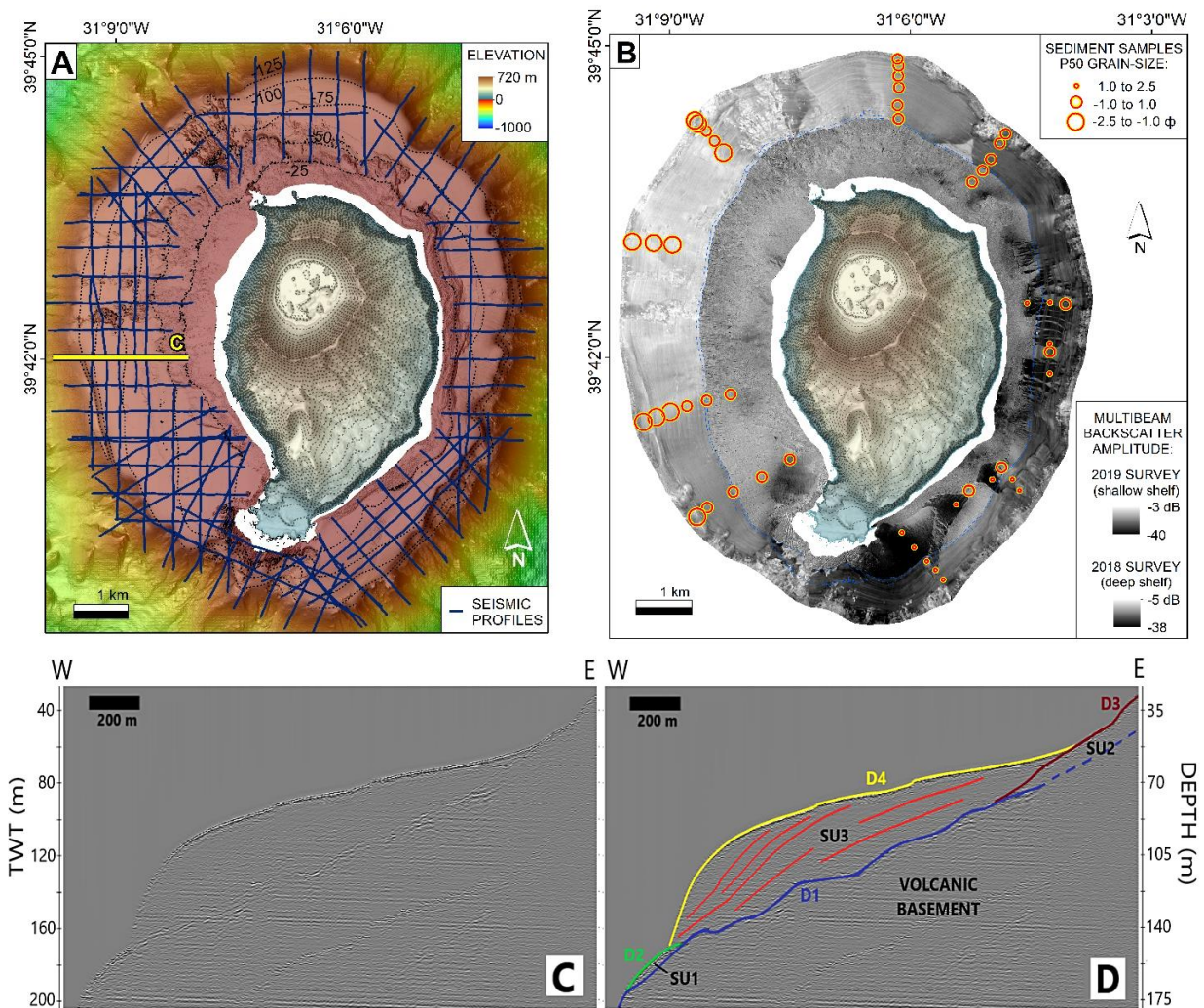
Figure 1. (A) Uninterpreted hillshade bathymetry and seismic profiles (blue lines) acquired at the insular shelf of Corvo. Yellow line locates seismic profile in (C) and (D). Thin dashed black contour lines are spaced every 25 m. (B) Multibeam backscatter mosaics of 2018 and 2019 on the same area. Lighter tones represent high backscatter values (in dB), while darker tones lower values (in dB). Orange circles mark sediment sample locations: circle size reflects median grain-size (D50 in \phi ). (C) Uninterpreted and (D) interpreted example of the E-W seismic profile, highlighted at (A). “TWT” = two-way times (in ms).
