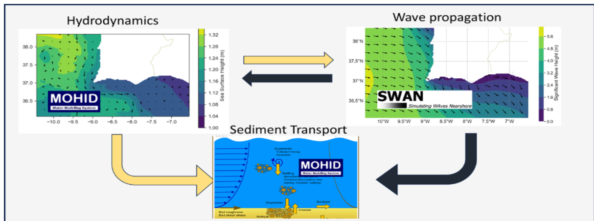
Figure 2. Numerical framework developed to assess oceanic risks on the wreck formed by three main components coupled: hydrodynamics, waves and non-cohesive sediment transport.
