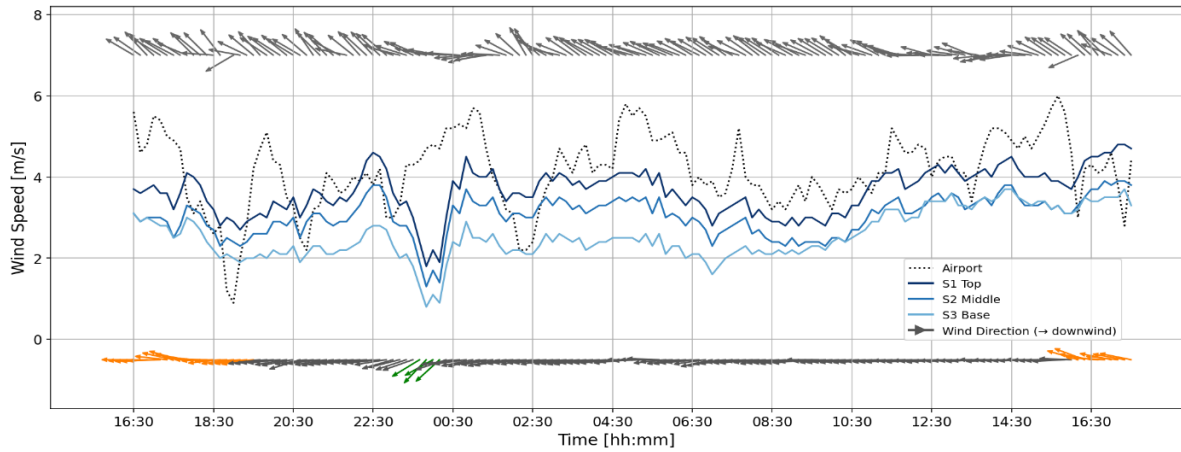
Figure 2. Top: time variation in airport wind direction. Middle: time variation of wind speed in airport, S1 to S3. Bottom: time variation in S1 direction.
