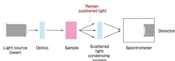
Figure 1. Common setup of Raman systems ( www.hamamatsu.com ).
