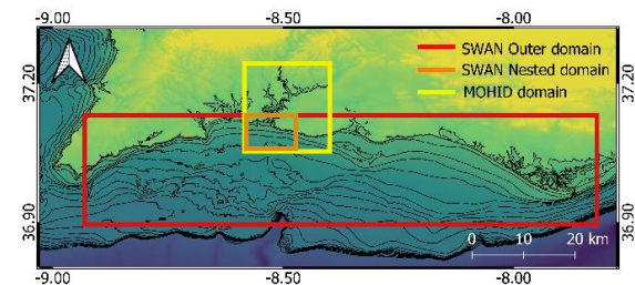
Figure 2. Map of numerical domains used for the wave simulations.
