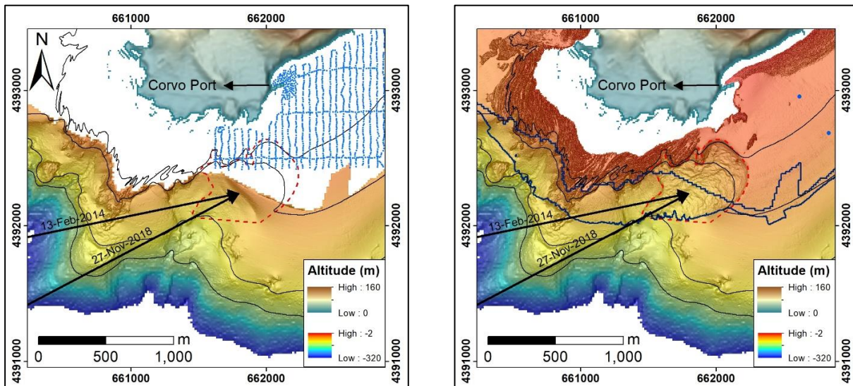
Figure 2. (A) Bathymetric data from 2000 (light-blue dots) and 2018 (colour ramp from blue to red), showing the landslide scar (dashed red line) and the approach directions of two storm waves (solid black arrows). Black contour lines indicate depths of 25, 50, 100, and 150 meters. (B) Merged bathymetric data from 2018 and 2019 (colour ramp from blue to red), with the overlapping survey area outlined in dark blue. Light blue dots represent the Smith MacIntyre grab samples.
