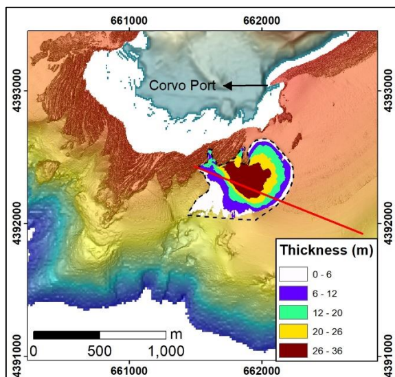
Figure 3. Thickness of displaced material from analysis of pre- and post-landslide bathymetry. Red line indicates the seismic profile location in Figure 4.
