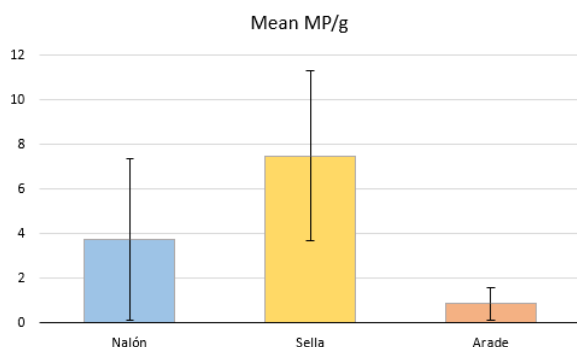
Figure 3. Comparison of the means ( \pm standard deviation) of MP concentration in limpets in the three studied estuaries: Nalón, Sella and Arade. Bars represent the mean values, and error bars indicate data variability.
