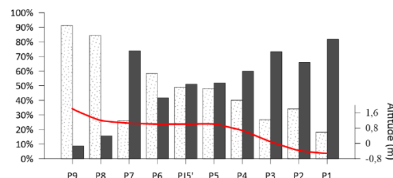
Figure 5. Percentage of sand (dots) and mud (dark grey) in sampling points (red line; topographic profile obtained with GSSN – datum Cascais).
