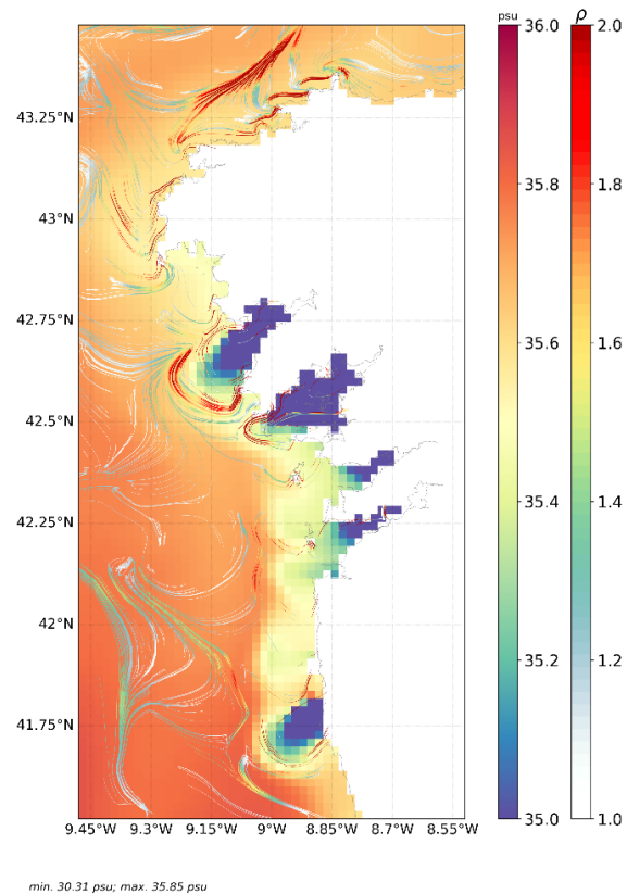
Figure 3. LCSs computed in ROMS model on 13/12/2023 between 16h and 21h and its salinity field on 13/12/2023 at 18h.
