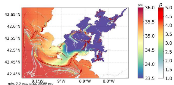
Figure 4. LCSs computed in MOHID Arousa model on 11/12/2023 between 10h and 16h and its salinity field on 11/12/2023 at 10h.
