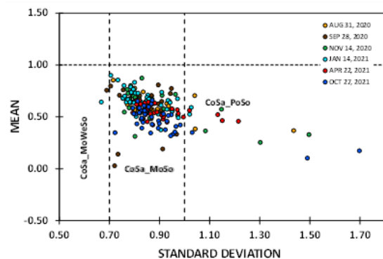
Figure 4. Mean versus standard deviation of native sediment collected in the various sampling campaigns (moments method).
