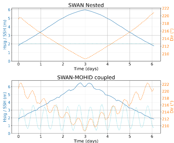
Figure 4. Comparison of simulated wave characteristics by the SWAN Nested model (top) and the coupled SWAN-MOHID model (bottom), showing significant wave height (Hsig), sea surface height (SSH) and wave direction (Dir), at the mouth of the estuary.
