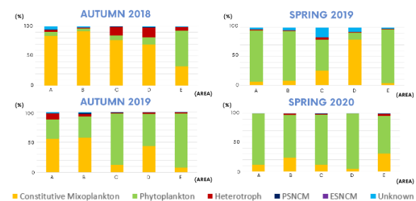
Figure 2. Percentage of abundance of the different trophic groups in the studied areas (A to E) for each campaign.
