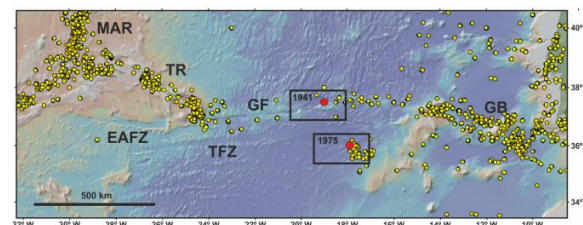
Figure 1. Study areas (black rectangles) and location of earthquakes. Yellow dots correspond to the location of earthquakes with M_w \geq 4.5 and red dots correspond to the epicenters of 1941 and 1975 events (catalogues USGS and SHARE). MAR: Mid-Atlantic Ridge; TR: Terceira Rift; EAFZ: East Azores Fracture Zone; GF: Gloria Fault; TFZ: Tydeman Fracture Zone; GB: Gorringe Bank.
