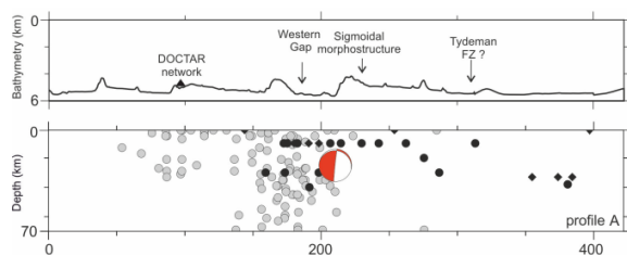
Figure 4. Profiles A across the seismicity cluster around the epicenter of the 1941 earthquake. Top: bathymetric profile. Bottom: depth projection of the earthquakes and micro-earthquakes. The focal mechanism of the 1941 events is also shown.
