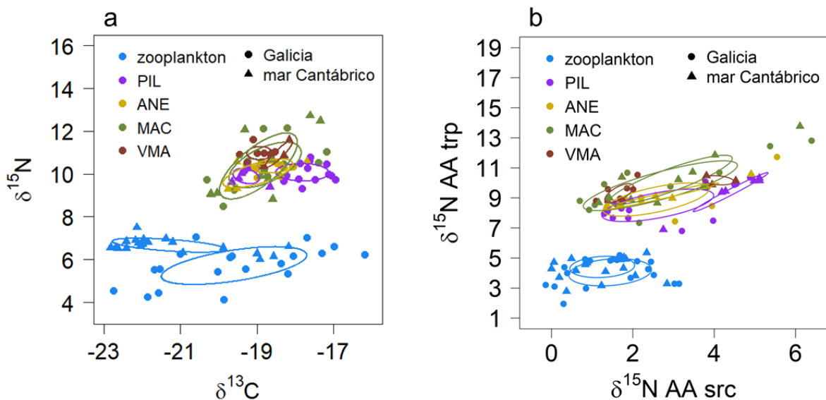
Figure 2. Standard ellipses for zooplankton and fish species determined by (a) bulk \delta^{15}\text{N} and \delta^{13}\text{C} values or (b) \delta^{15}\text{N} values in trophic ( \delta^{15}\text{N}_{\text{trp}} ) and source ( \delta^{15}\text{N}_{\text{src}} ) amino acids (AA) in Galicia and mar Cantábrico study areas. PIL: Sardina pilchardus , ANE: Engraulis encrasicolus , MAC: Scomber scombrus , and VMA: Scomber colias .
