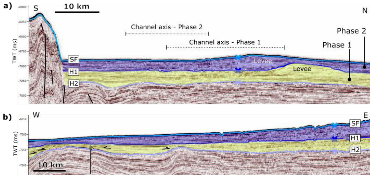
Figure 2. a) Seismic profile perpendicular to the distal channel and fan, highlighting the sequences of the interpreted Phase 1 and Phase 2. The limits of the channel axis for each phase are shown, indicating a southward shift of the system. b) seismic section along the length of the fan, showing Phase 1 sequences infilling paleoreliefs and onlapping onto folds. Phase 2 deposits as a west-thinning wedge.
