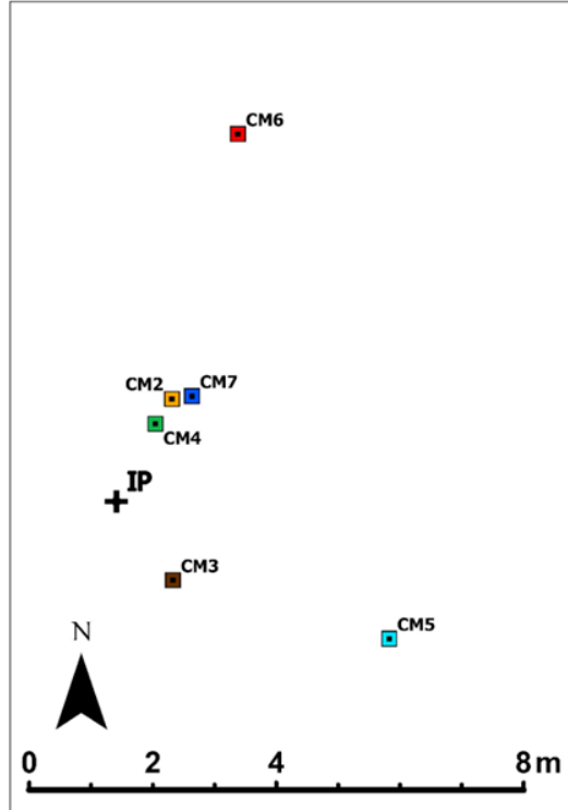
Figure 5. Positions occupied by the successive centers of mass of the tracer (CM2 to CM7). Note: the center of mass for the first sampling campaign (CM1) is not represented because no tracer particles were detected. IP – Injection point. Each color represents a different sampling interval being correspondent to the colors used in Figure 1.
