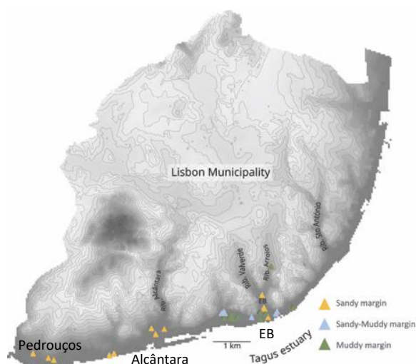
Figure 3. Location of sediments collected in the Lisbon estuarine margin in salvage archaeological works.
