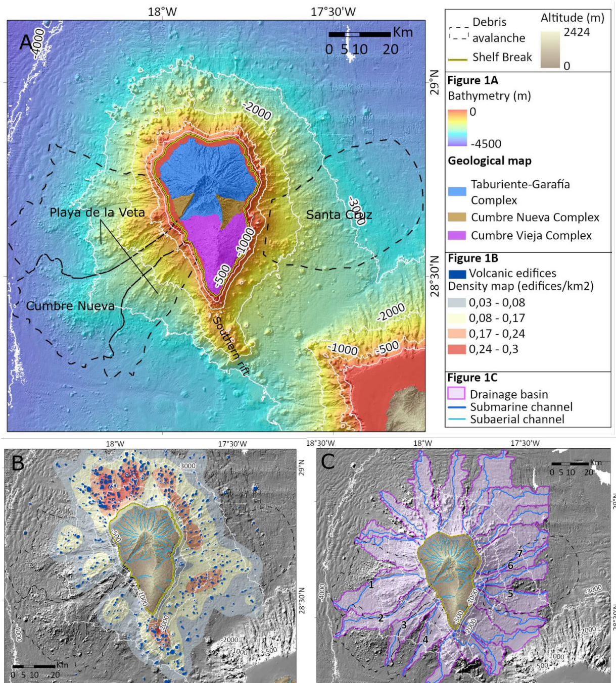
Figure 1. A) Bathymetric and simplified geological map of La Palma. The black dashed line indicates mass transport deposits (Masson et al. , 2002). ; B) Density map of volcanic edifices surrounding the island of La Palma; C) Drainage basins boundaries and main drainage channels of La Palma. The well-defined canyons are numbered from 1 to 7.
