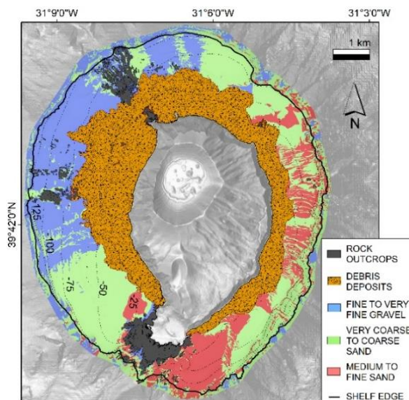
Figure 4. Seafloor characterization of Corvo's insular shelf.
